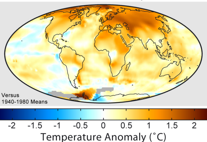
1999-2008 Mean Temperatures
